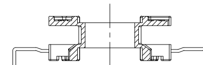
SECTION C-C
